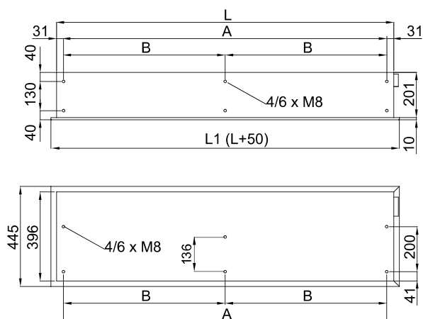
Control Panel (*)
